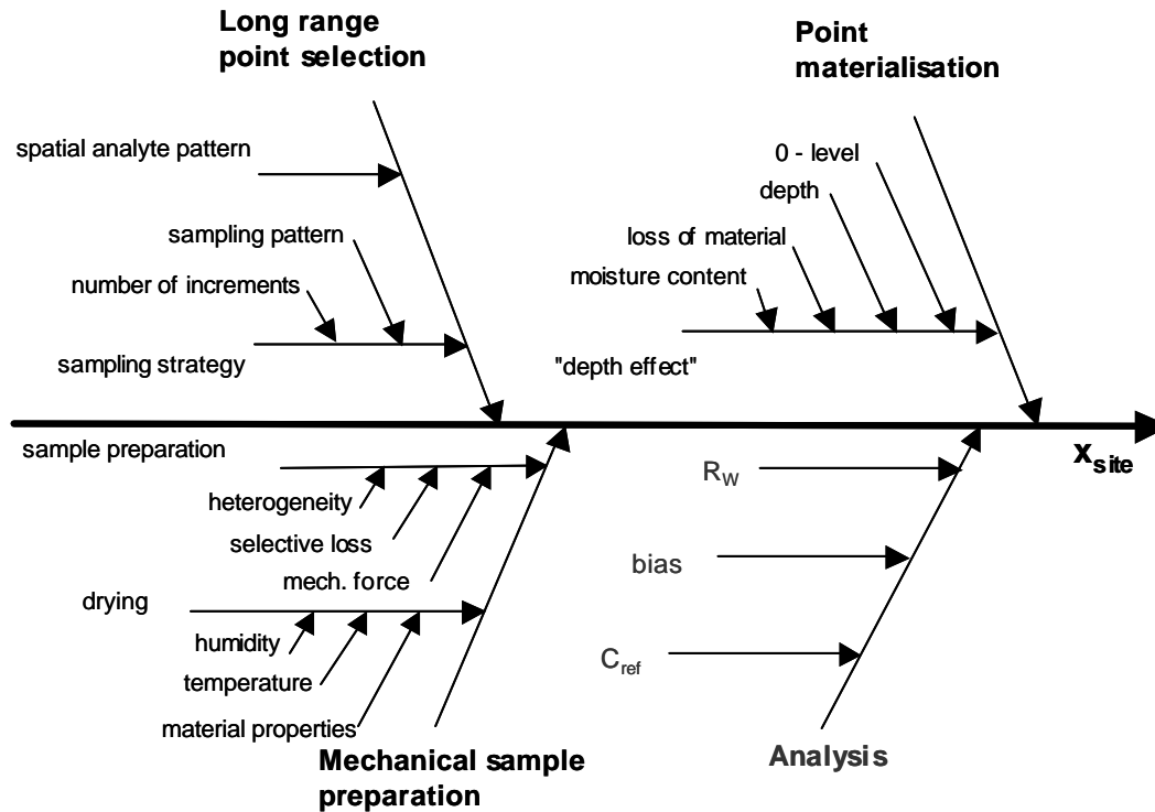
Figure A6.1: Cause & effect diagram for soil sampling on arable land ( R_w is within-laboratory reproducibility)
